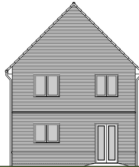
Rear Elevation
